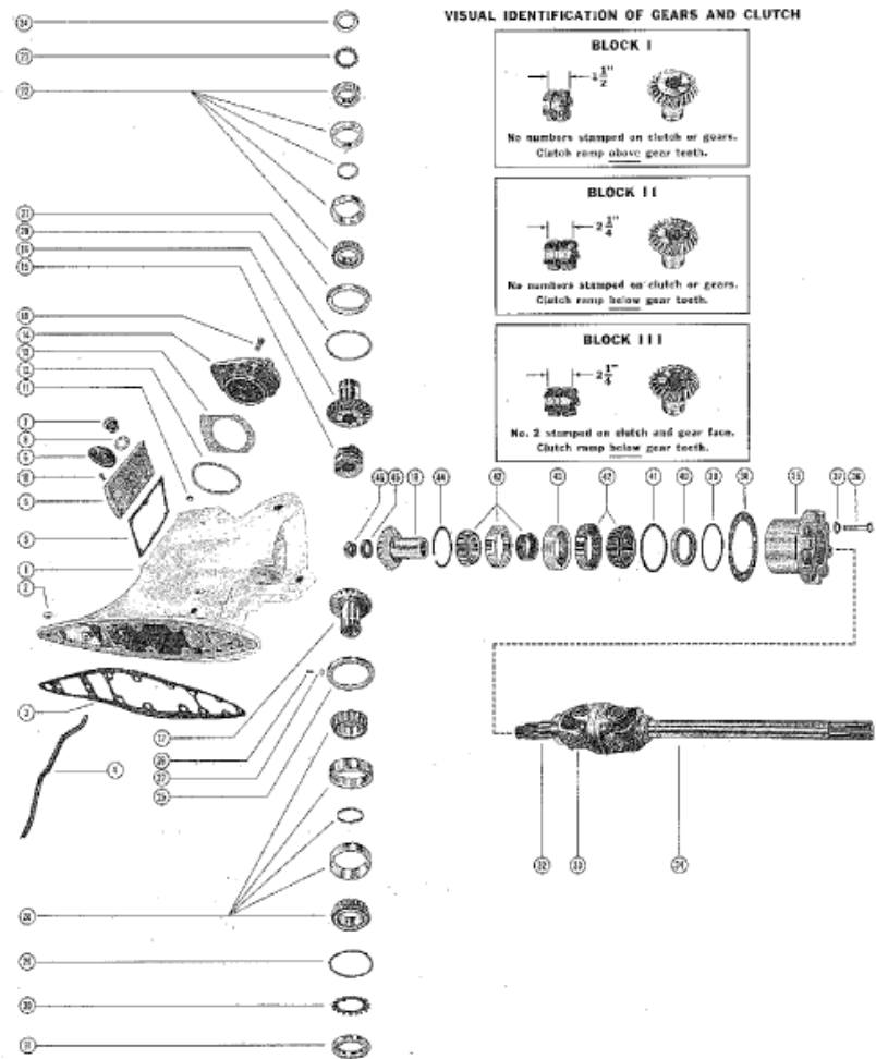
VISUAL IDENTIFICATION OF GEARS AND CLUTCH
