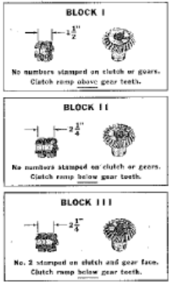
VISUAL IDENTIFICATION OF GEARS AND CLUTCH
